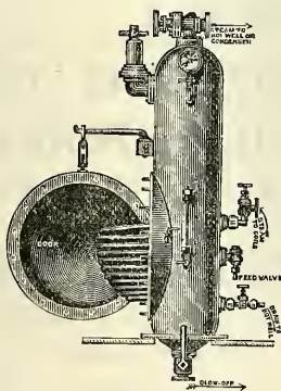
EVAPORATOR.
