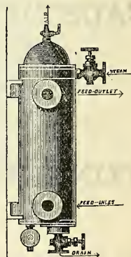
HEATER.
