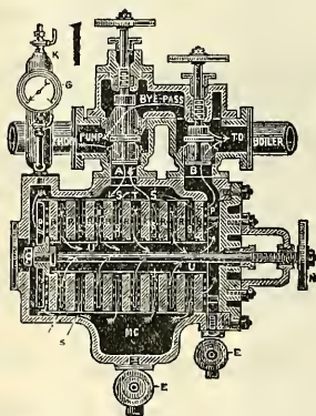
FILTER.
