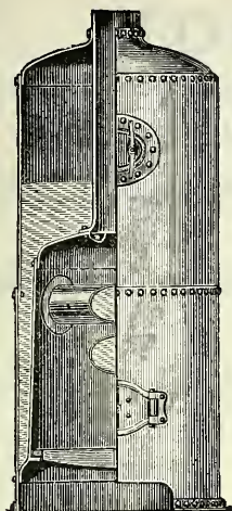
Vertical Cross-Tube Boiler.
