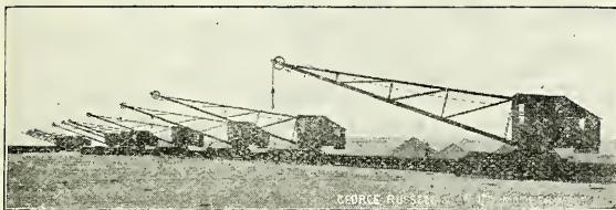
Electric Cranes on Roof of Transit Shed, Salford Docks.
