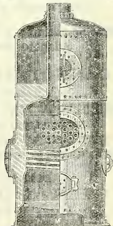
Simplex Vertical Boiler.
