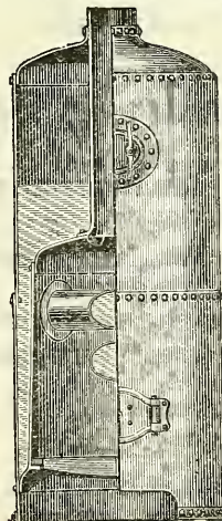
Vertical Cross-Tube Boiler.
