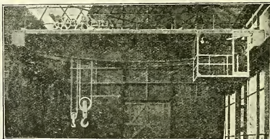
30-Tons Four-Motor Electric Crane.
