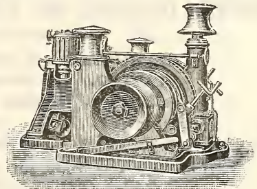
Steam Windlass for Yachts.
