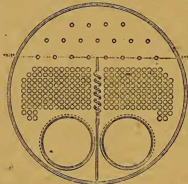
SECTION OF BOILER SHOWING “BEAVER” CIRCULATOR BETWEEN THE TUBES.
